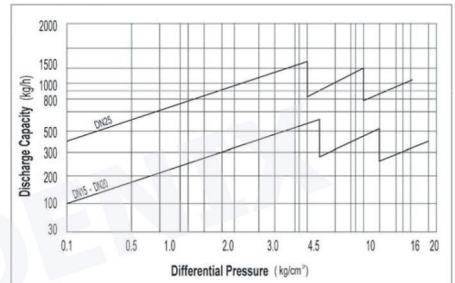
Discharge Capacity
