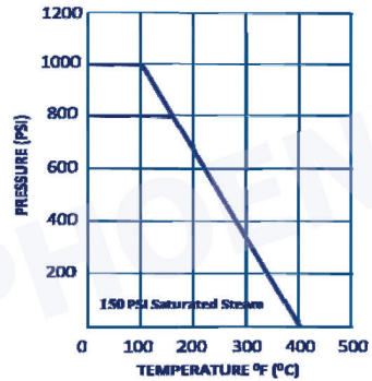
PRESSURE / TEMPERATURE RATING
